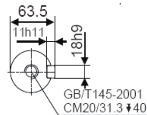
Polar Wind - 5 Mounting Pattern
